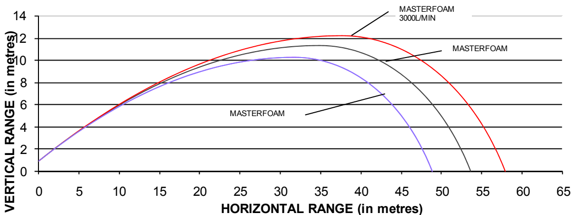
RANGE of MASTERFOAM NOZZLES at 7 BAR with FOAM at 3%
